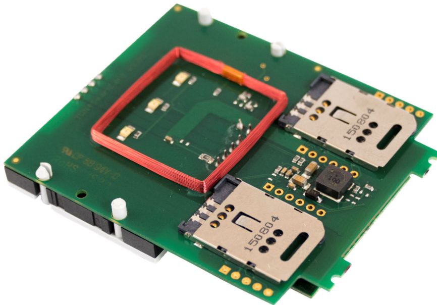
PCB contained in TWN4 MultiTech SmartCard LEGIC 42
